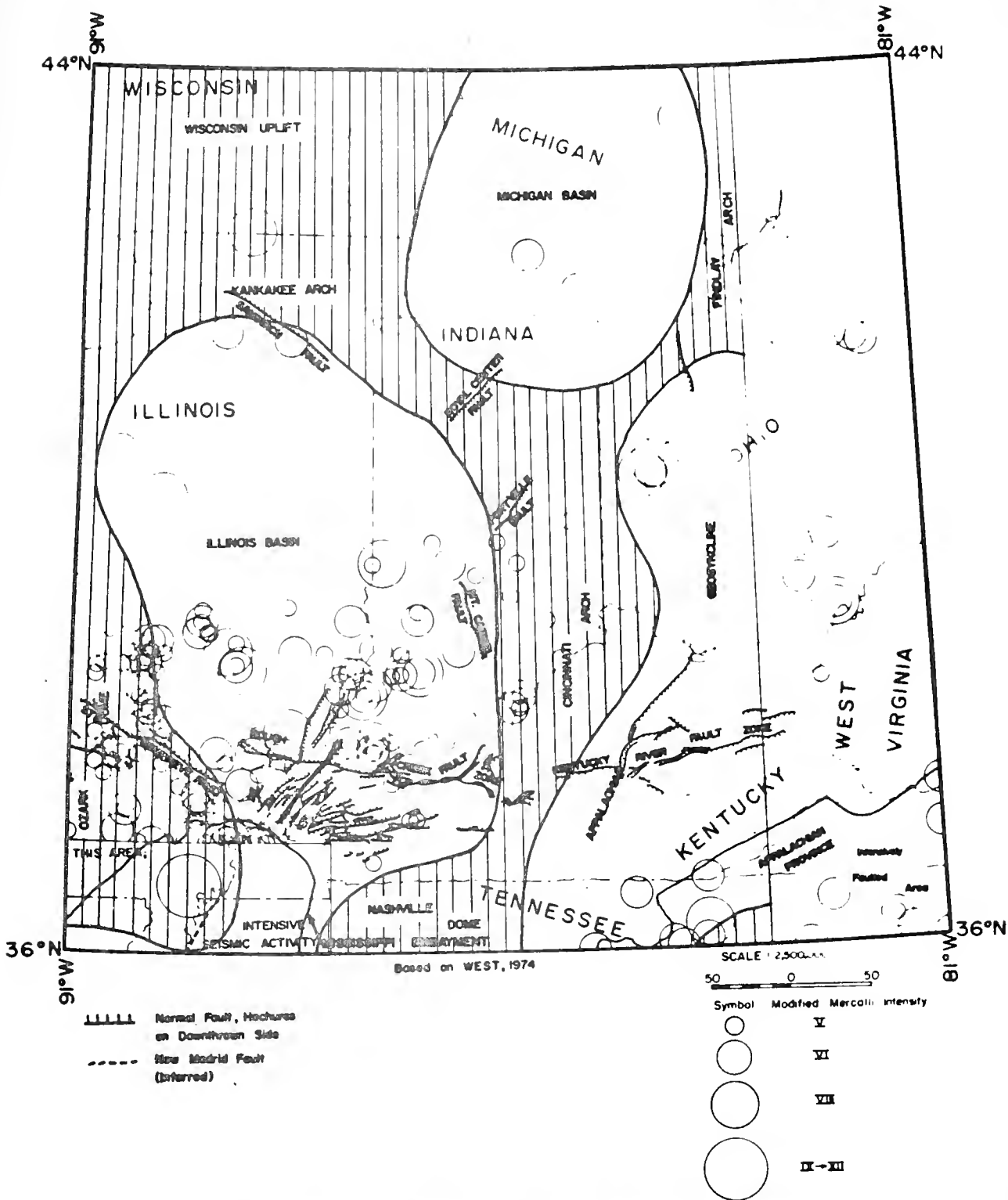
FIGURE 8 REGIONAL TECTONIC MAP.
